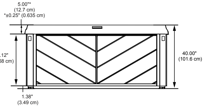
SIDE VIEW Tolerance: \pm 0.5" (1.27 cm)
