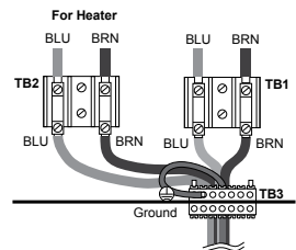
Double Breaker Connection
