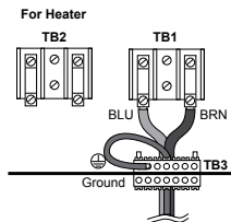
Single Breaker Connection
